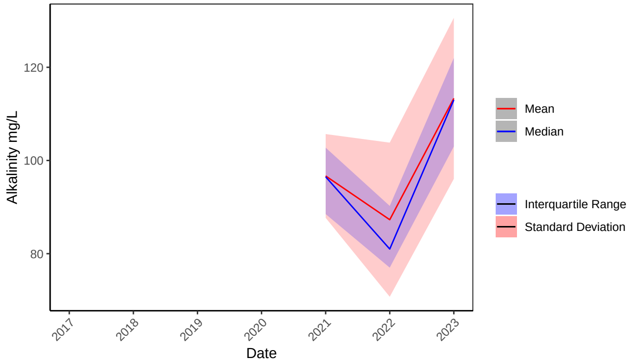
B2 Raceway 2 Alkalinity mg/L Yearly Statistics
